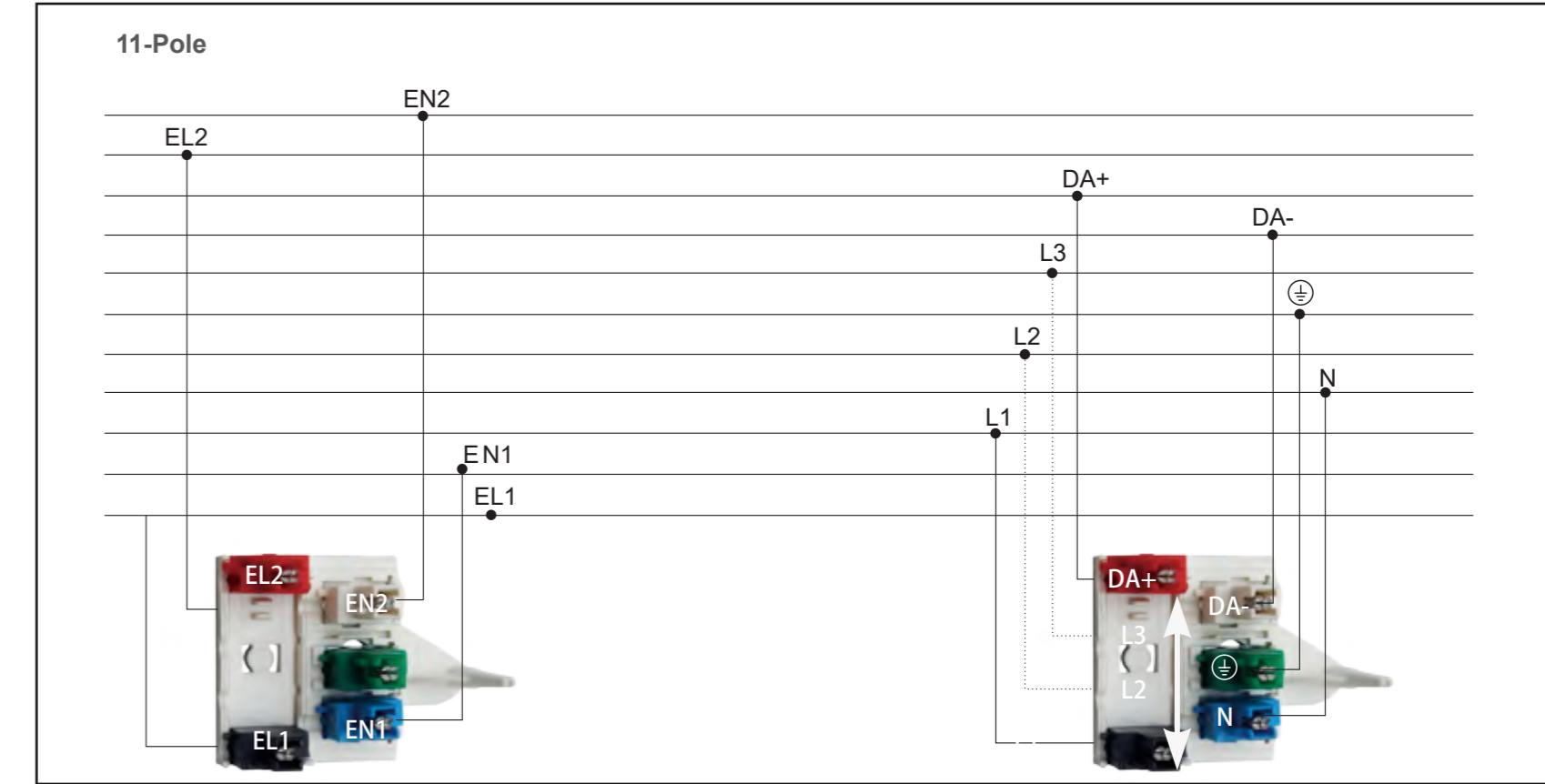
11-Pole
